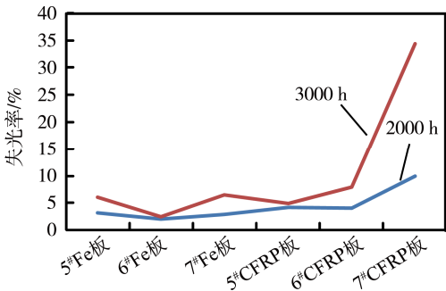
图 3 样品在不同基材上 2000 h 和 3000 h 失光率对比 Fig.3 Comparison of the rate of loss of light in 2000 h/3000 h of samples at different substrate
