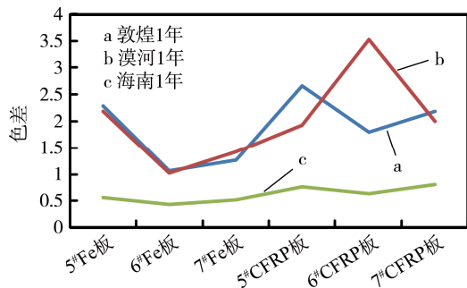
图 6 样品在不同基材上国内试验站色差对比 Fig.6 Comparison of the aberration in domestic experimental stations of samples at different substrate
